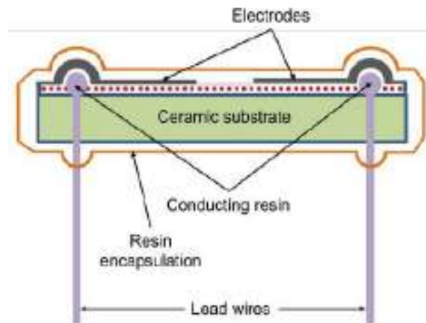
Fig 1: Construction of Light Sensors
