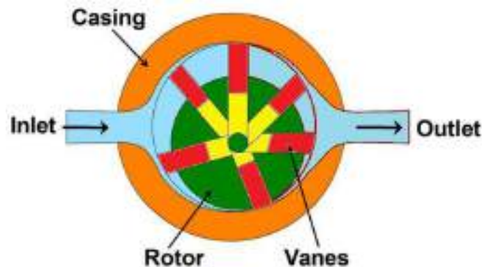
Fig. 5.1.3 Rotary vane compressor
