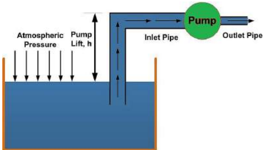
Figure 5.4.4 Pump lift
