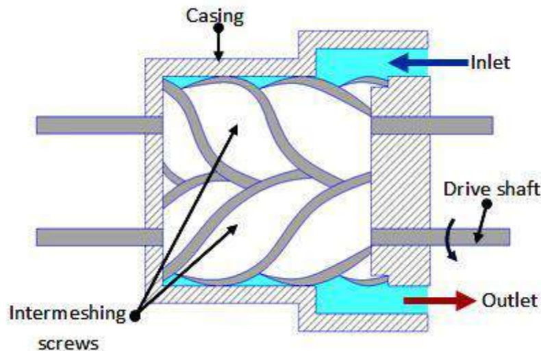
Fig. 5.1.2 Screw compressor
