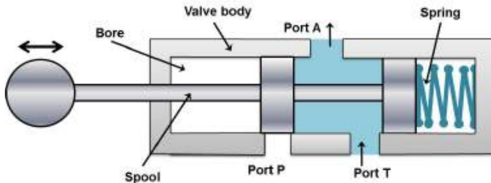
Figure 5.2.8 Three way valve in closed position
