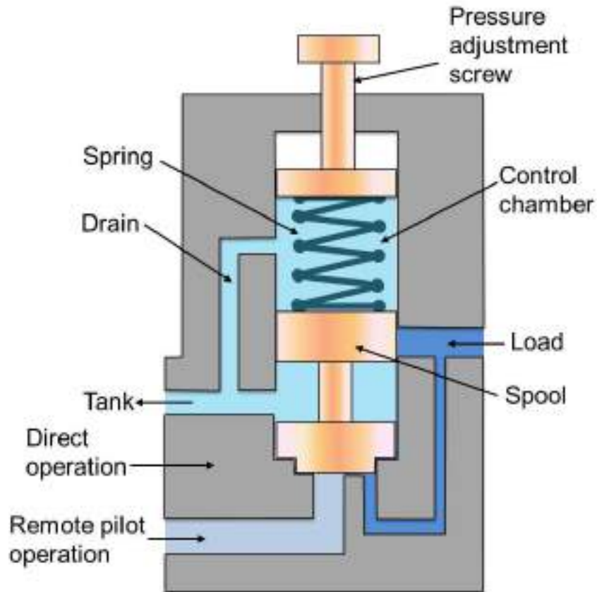
Figure 5.2.29 Counter Balance Valve
