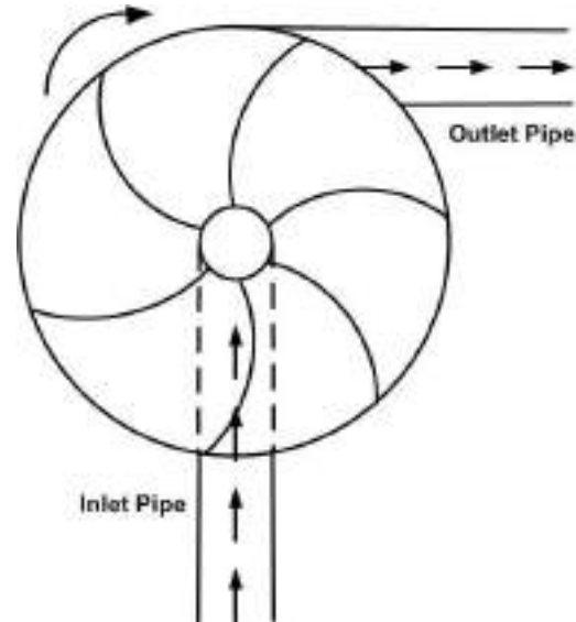
Figure 5.4.3 Centrifugal pump
