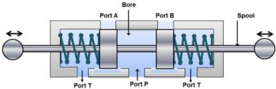
Figure 5.2.13 Tandem centered valve
