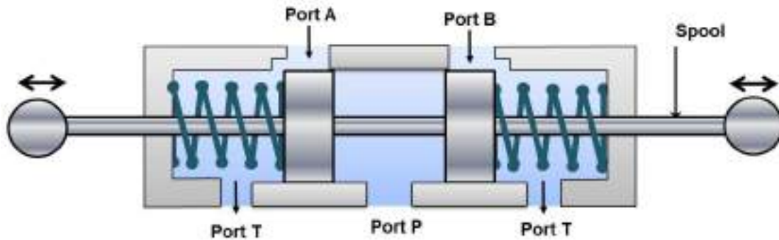
Figure 5.2.15 Floating Center
