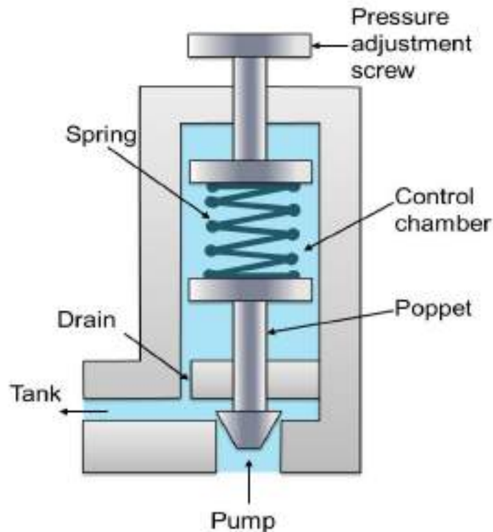
Figure 5.2.26 Pressure Relief Valve
