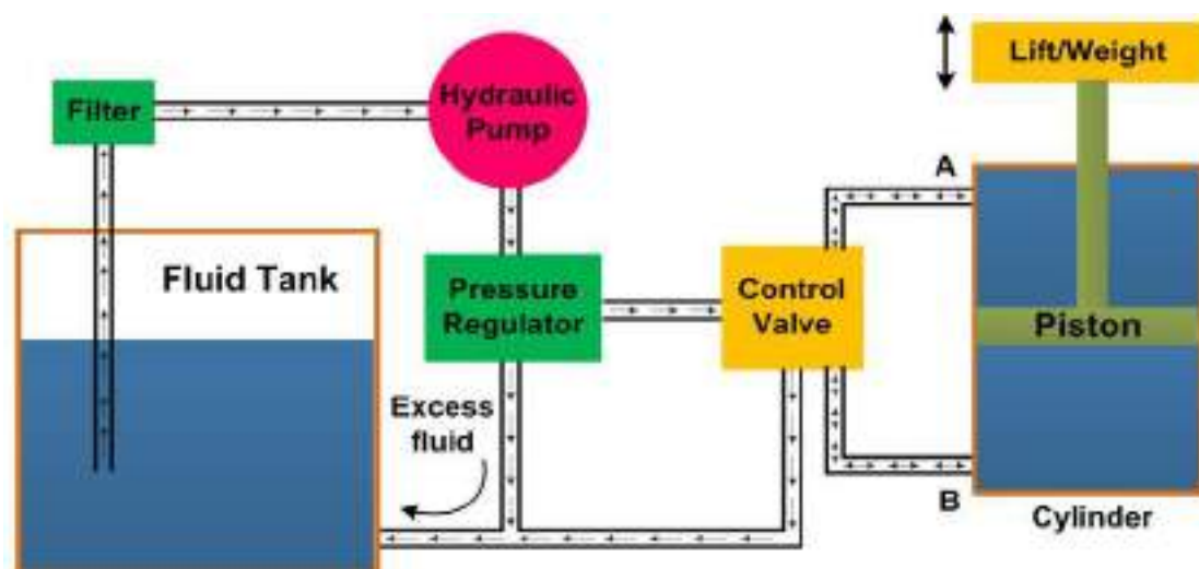
Figure 5.4.2 Schematic of hydraulic system
