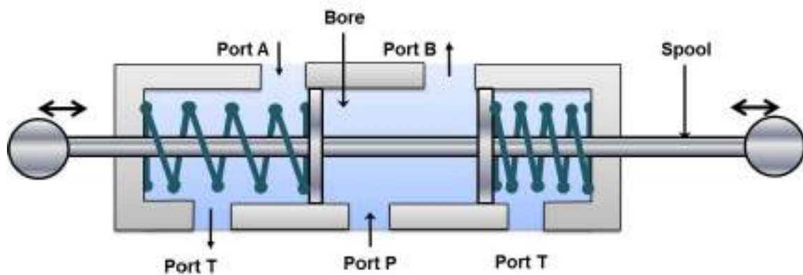
Figure 5.2.10 Three position four way valve: P to B and A to T
