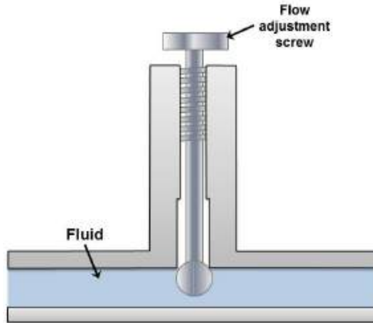
Figure 5.2.21 Flow Control Valve
