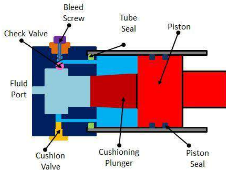
Fig. 5.3.3 Cylinder end cushioning
