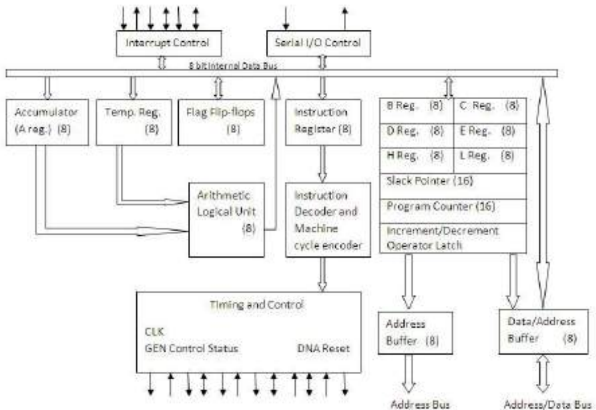
Figure 6 Architecture of 8085 microprocessor
