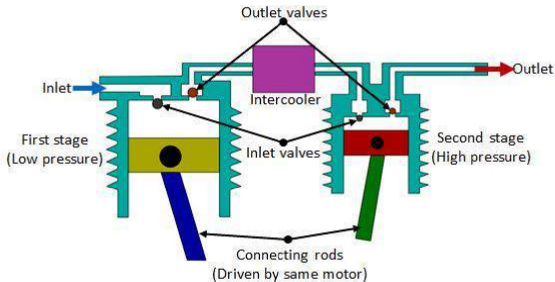
Fig. 6.1.5 Multi-stage compressor
