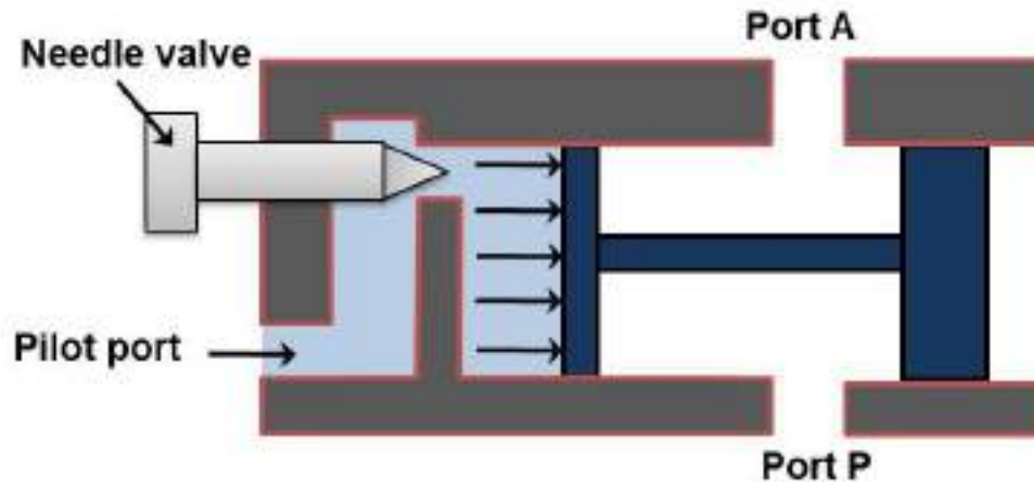
Figure 5.2.19 Pilot actuated DCV
