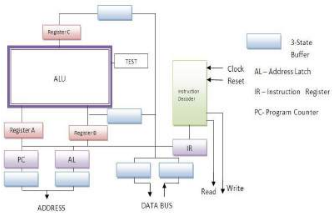
Figure 3 Working of a microprocessor
