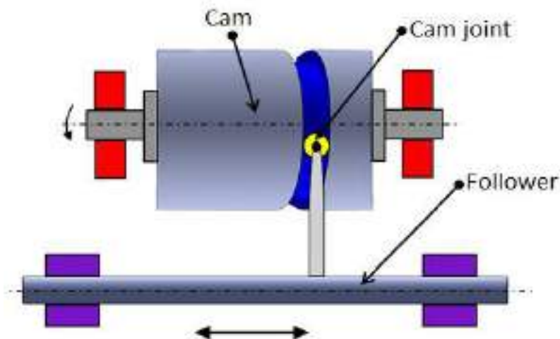
Figure 4.3.4 Cylindrical cam
