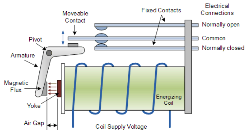
Fig 4.7.2: Relay
