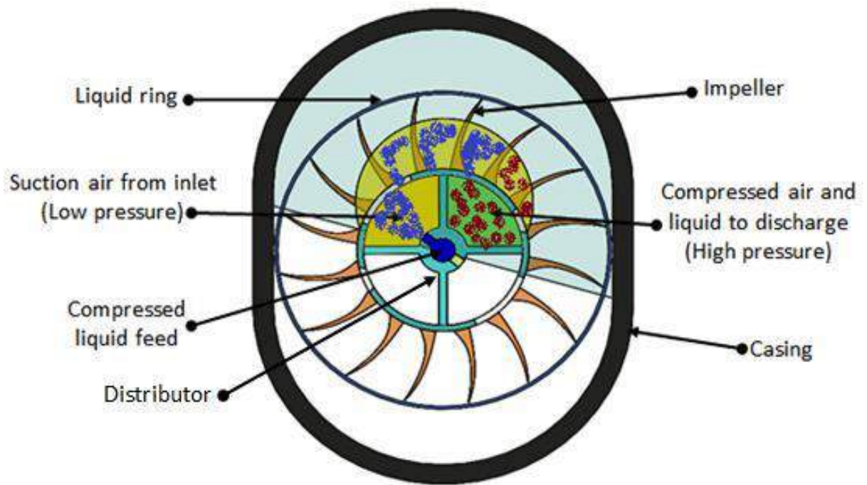
Fig. 5.1.4 Liquid ring compressor
