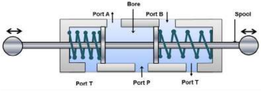
Figure 5.2.11 Three position four way valve: P to A and B to T
