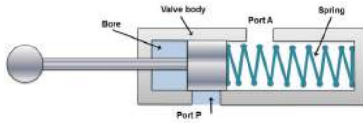
Figure 5.5.1 Valve closed
