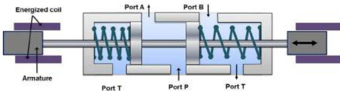
Figure 5.2.18 Working of solenoid to shift spool of valve
