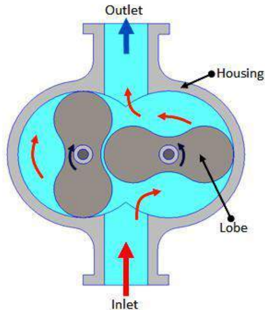
Figure 5.2.2 Lobe pump
