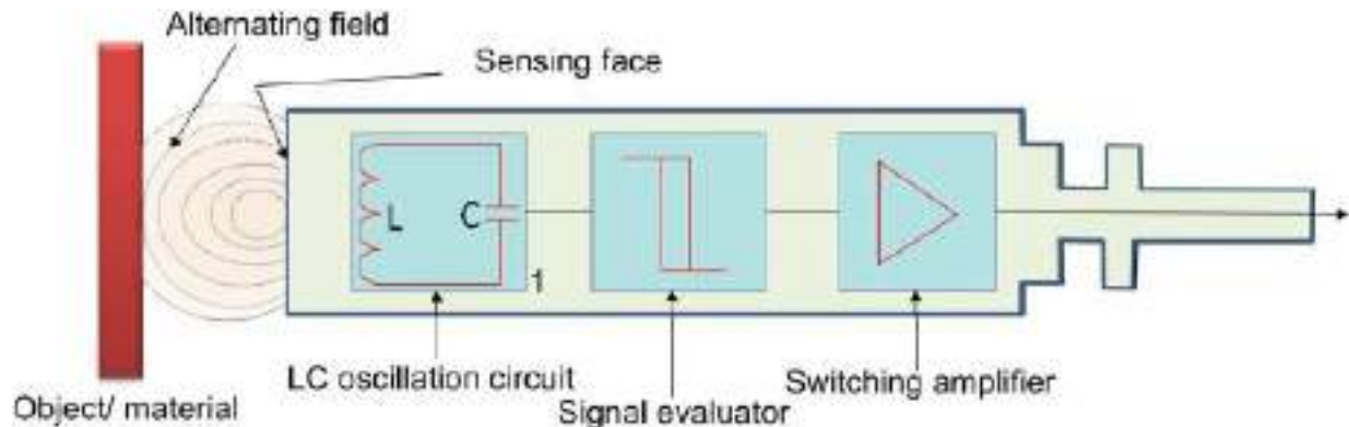
Fig 4: Schematic of Inductive proximity Sensor
