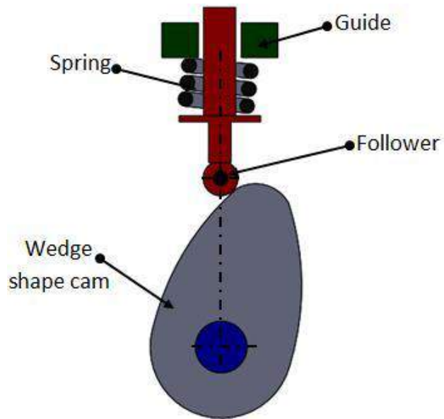
Figure 4.3.3 Plate cam
