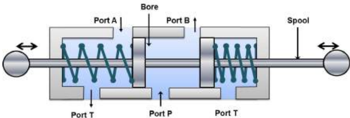
Figure 5.2.16 Two position four way DCV: P to B and A to T
