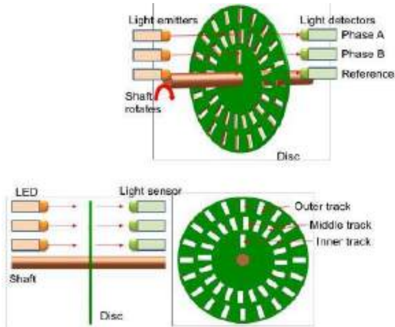
Fig 5: Construction and working principle of Optical Proximity Sensor
