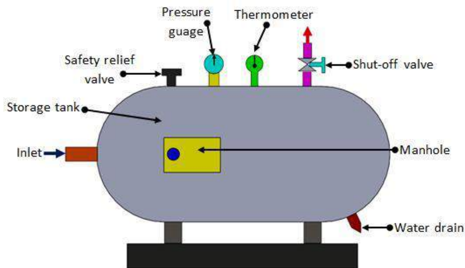
Fig.5.6.2 Air receiver
