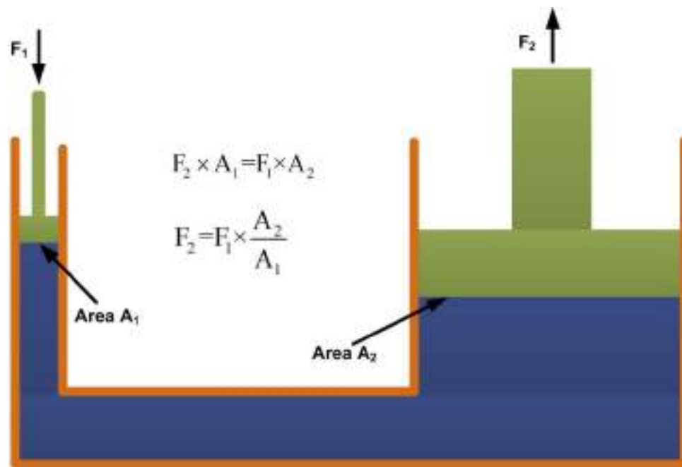
Figure 5.4.1 Principle of hydraulic system
