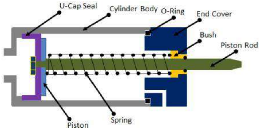
Fig. 5.3.1 Single acting cylinder
