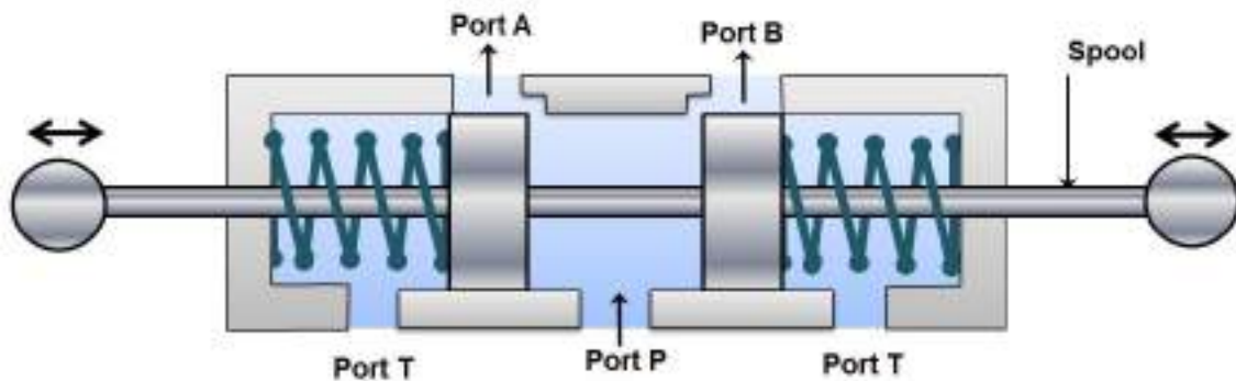
Figure 5.2.14 Regenerative Center
