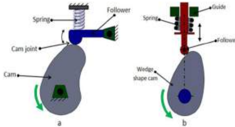
Figure 4.3.8 Force closed cam followers
