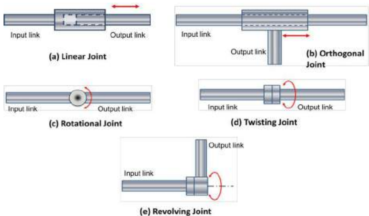
Fig. 3.5.2 Types of Joints
