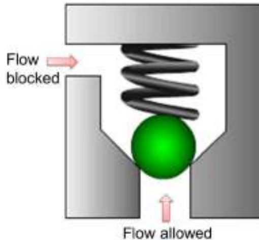
Figure 5.2.2 Right angle check valve
