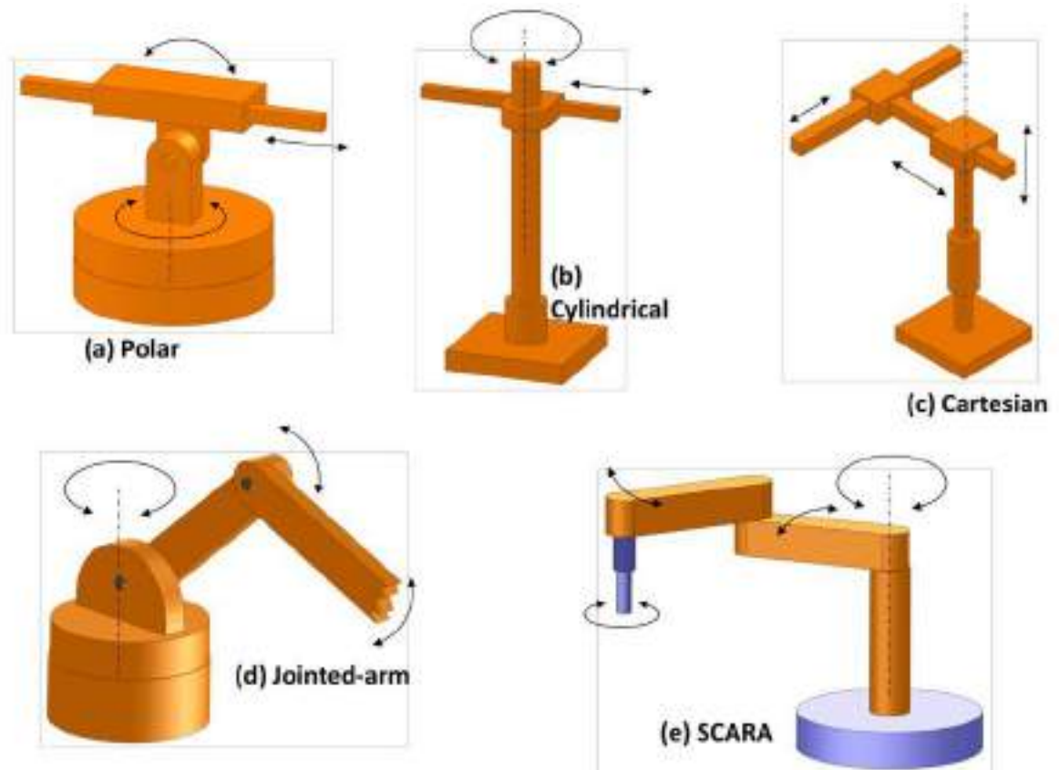
Fig.3.5.3 Common Body-and-Arm configurations
