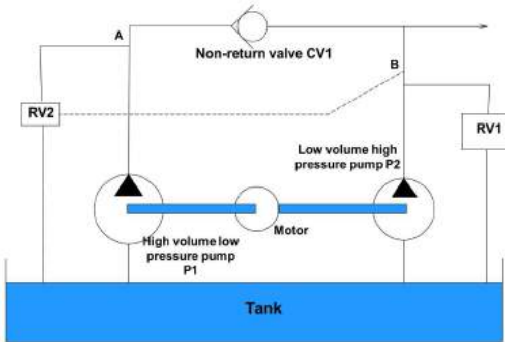
Figure 5.3.8 Combination pump
