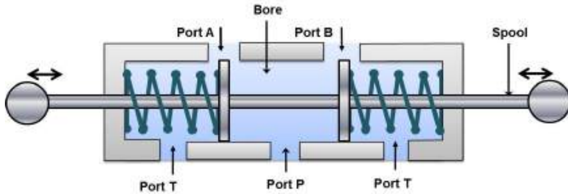
Figure 5.2.9 Three position four way valve in open center mode
