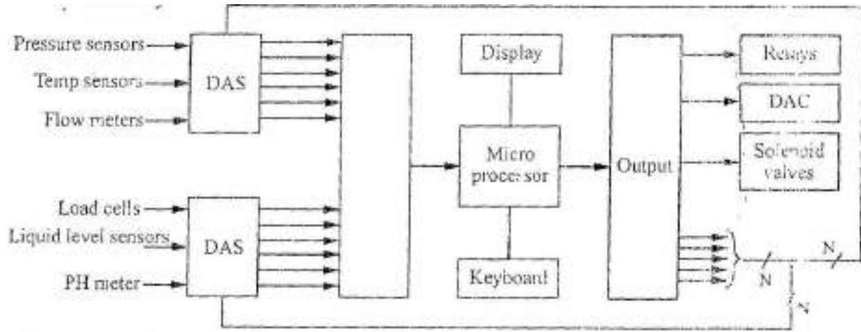
Fig 9: Microprocessor based control system
