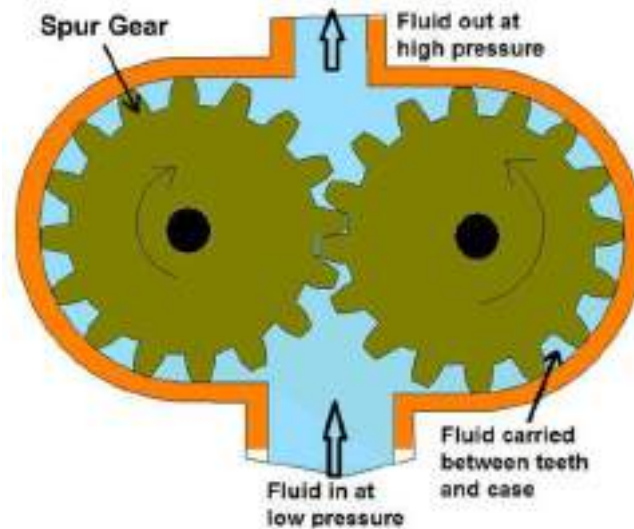
Fig. 5.3.4 Gear motor
