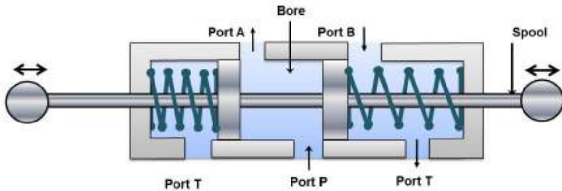
Figure 5.2.17 Two position four way DCV: P to A and B to T
