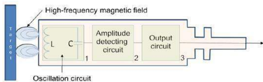
Fig 3: Construction of Eddy current proximity sensors
