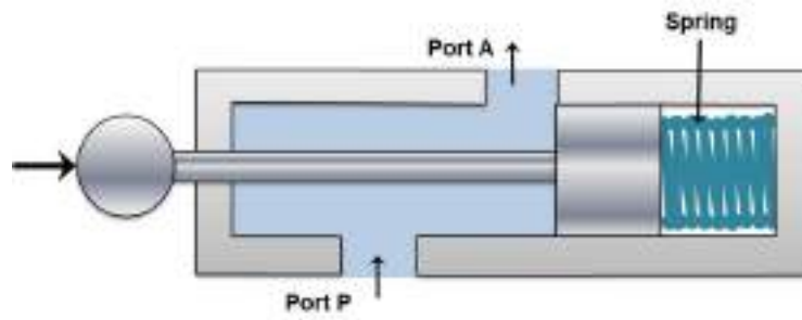
Figure 5.5.1 Valve closed
