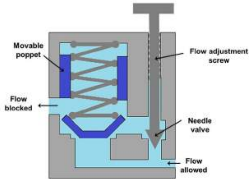
Figure 5.2.3 Restriction check valve
