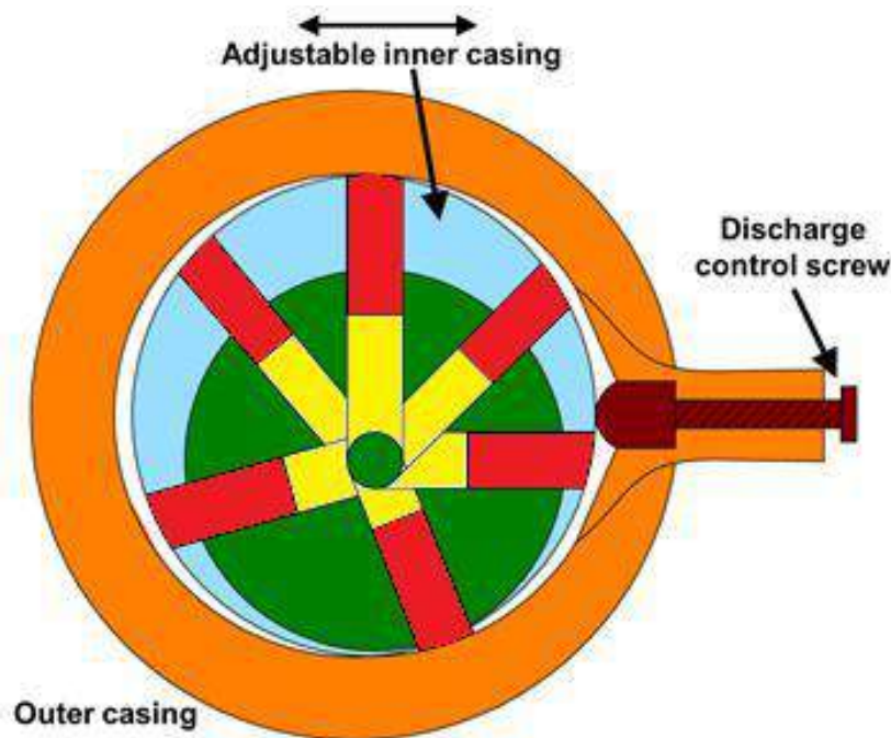
Figure 5.3.3 Adjustable vane pump
