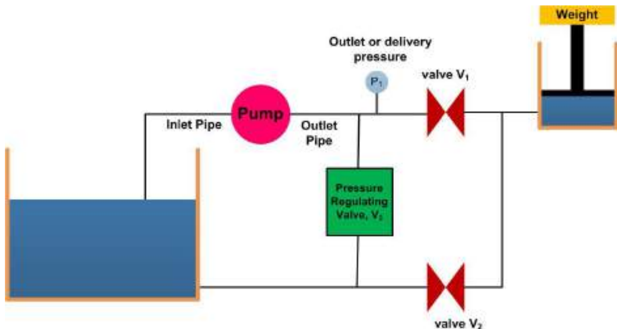
Figure 5.4.5 Schematic of pressure regulation
