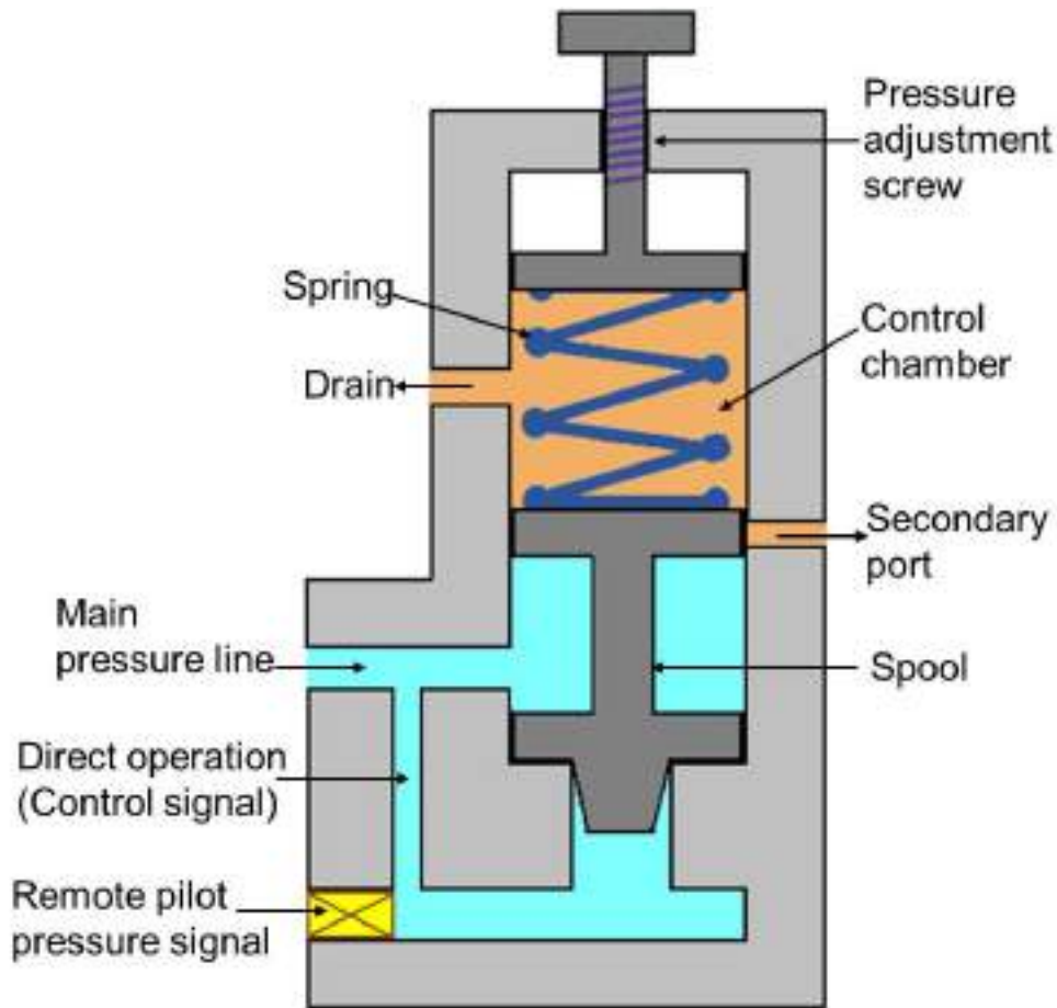
Figure 5.2.28 Sequence valve
