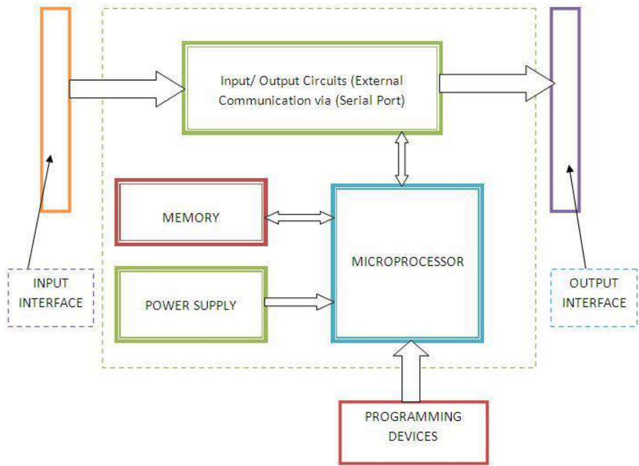
Figure 3.2.1 Block diagram of a PLC
