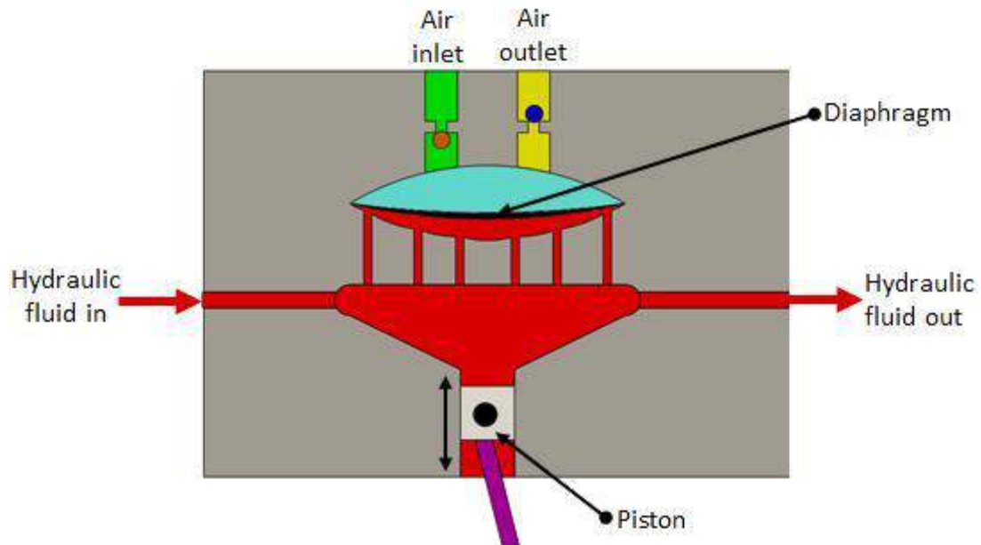
Fig. 5.1.1 Diaphragm compressor
