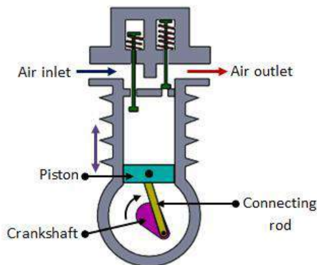
Fig. 5.6.3 Single acting piston compressor
