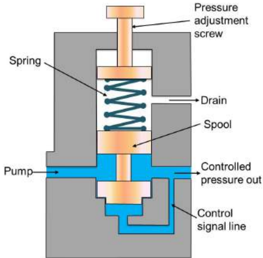
Figure 5.2.30 Pressure Reducing Valve
