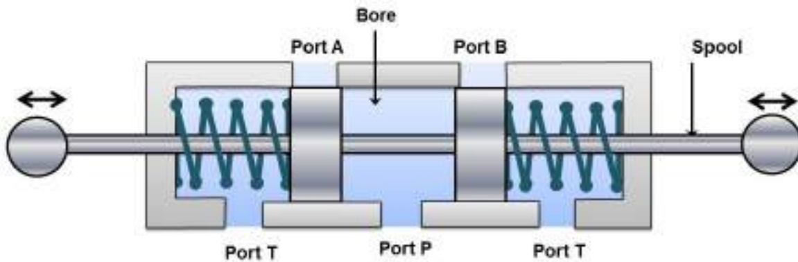
Figure 5.2.12 Three position four way valve: closed center
