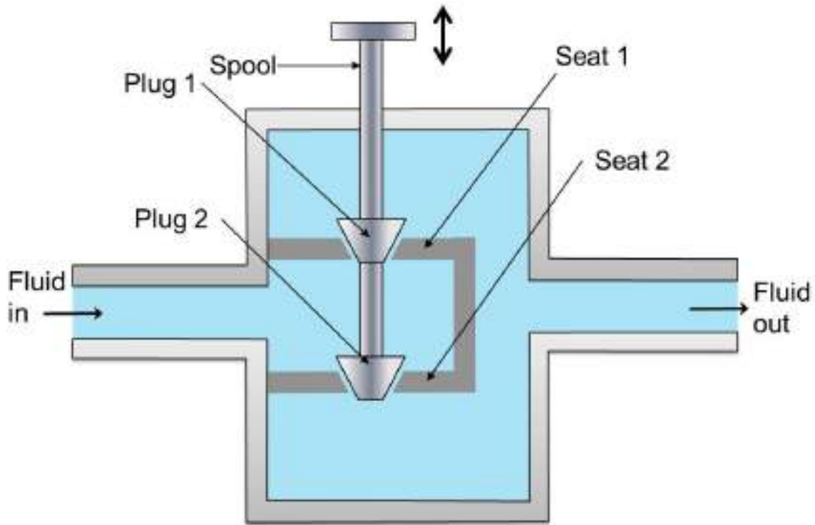
Figure 5.2.25 Balanced valve
