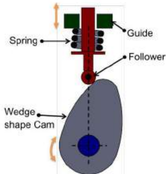
Figure 4.3.1 Cam mechanism.
