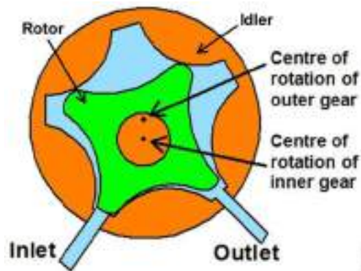
Figure 5.2.4 Gerotor pump
