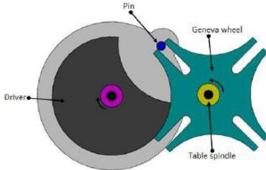
Fig. 4.5.3 Geneva mechanism
