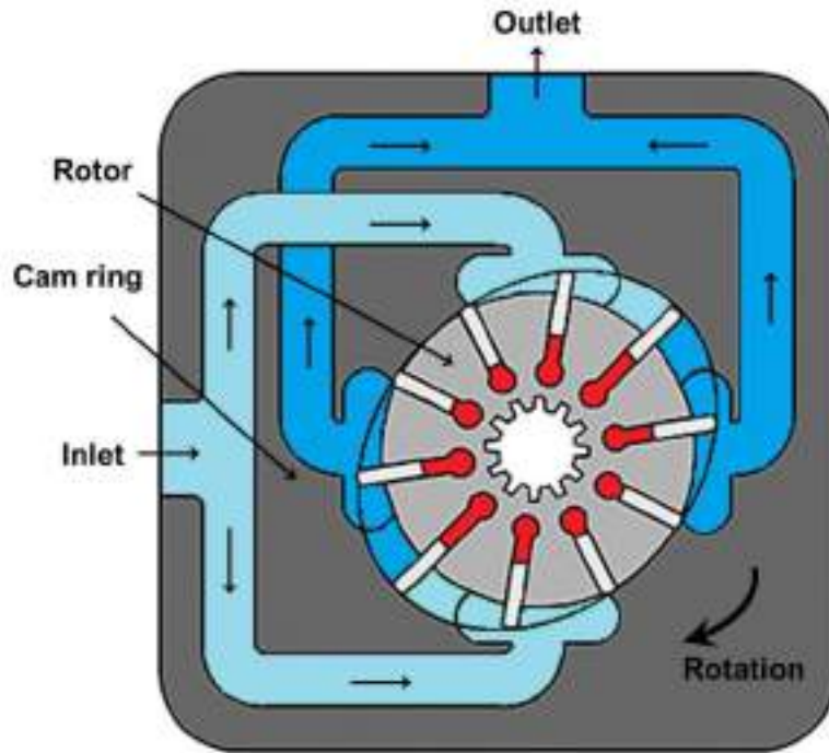
Figure 5.3.2 Balanced Vane Pump
