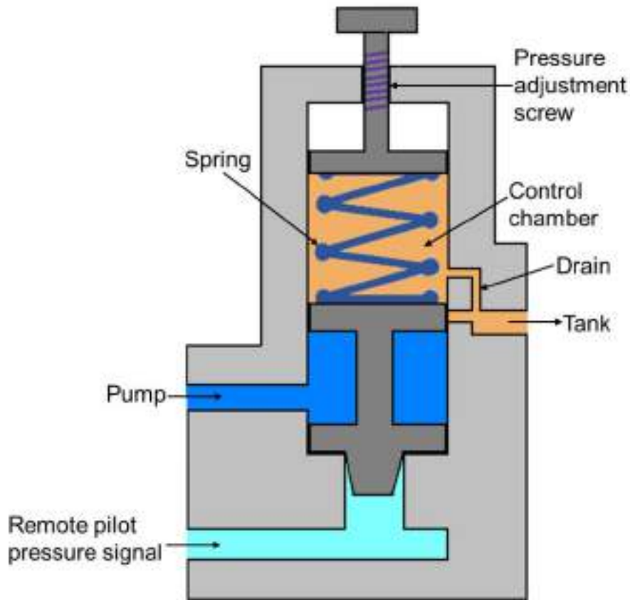
Figure 5.2.27 Unloading Valve
