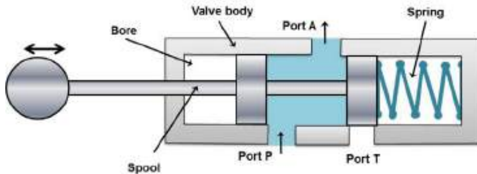
Figure 5.2.7 Three way valve: P to A connected and T is blocked
