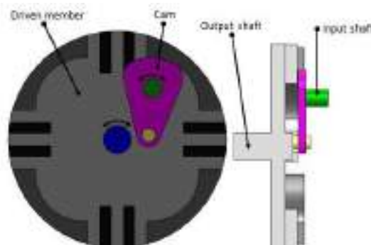
Fig. 4.5.4 Internal Geneva mechanism
