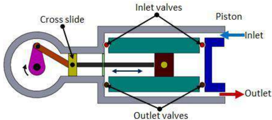
Fig. 5.6.4 Double acting piston compressor
