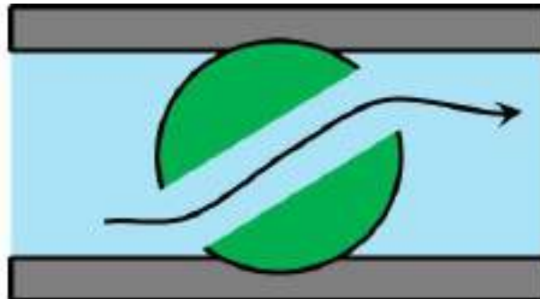
Figure 5.2.24 Ball valve
