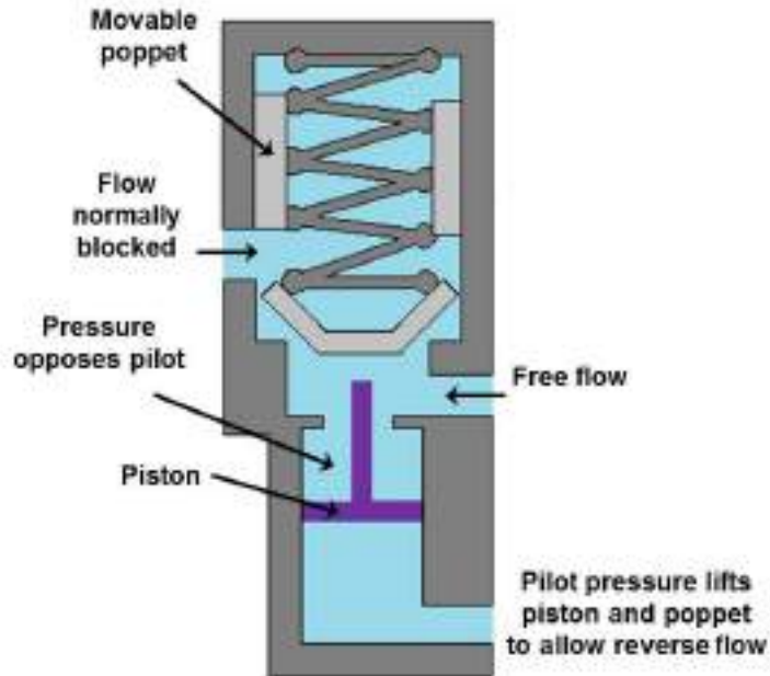
Figure 5.2.4 Pilot operated check valve
