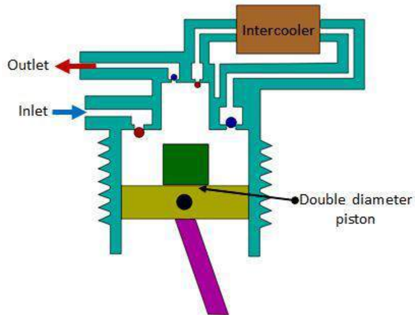
Fig. 5.6.6 Combined two stage compressor
