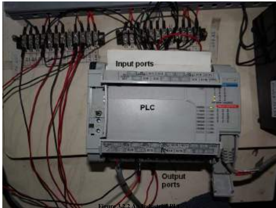
Figure 3.2.2 An Industrial PLC
