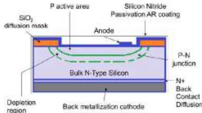
Fig 2: Construction of Photo diodes
