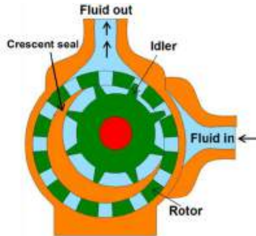
Figure 5.2.3 Internal gear pump
