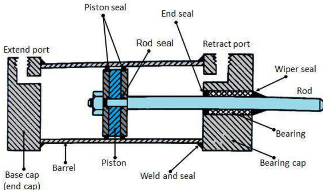
Fig. 5.3.2 Double acting cylinder
