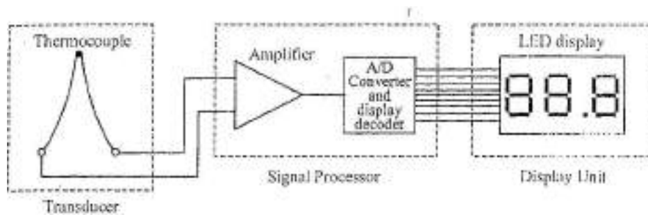
Fig 3: Digital thermometer principle
