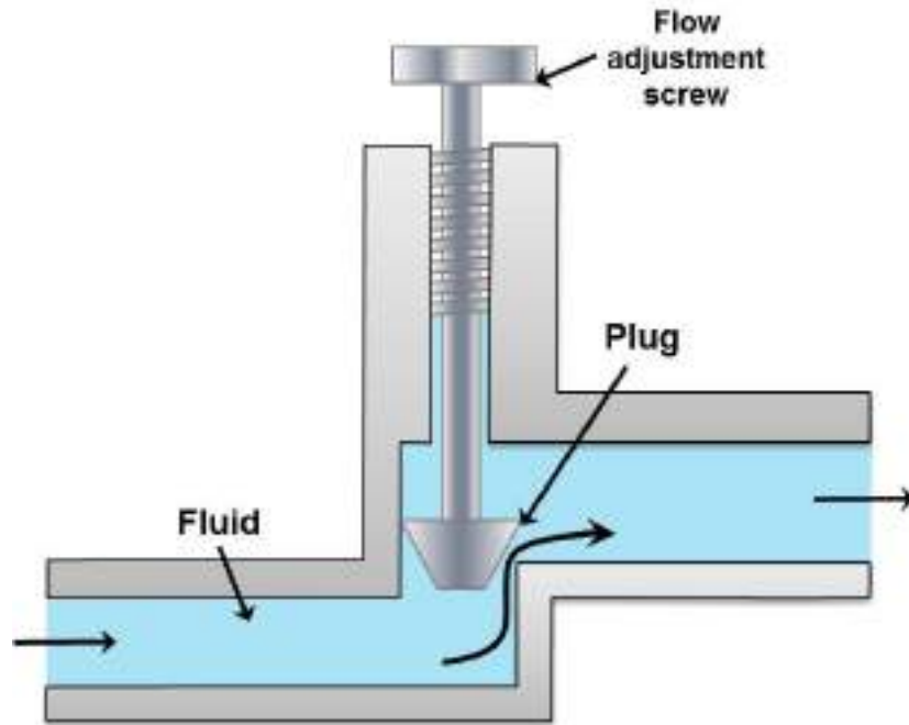
Figure 5.2.22 Plug or glove valve
