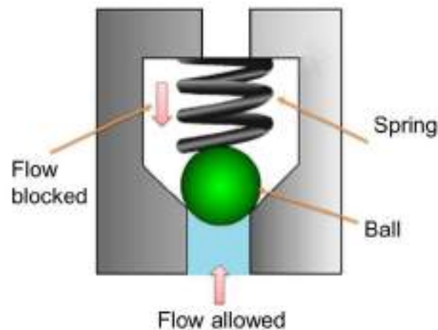
Figure 5.2.1 Inline check valve
