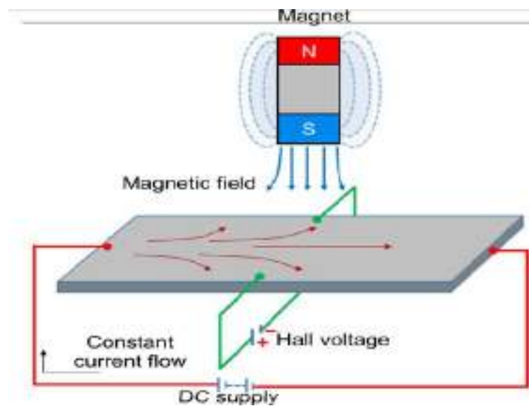
Fig 6: Hall Effect
