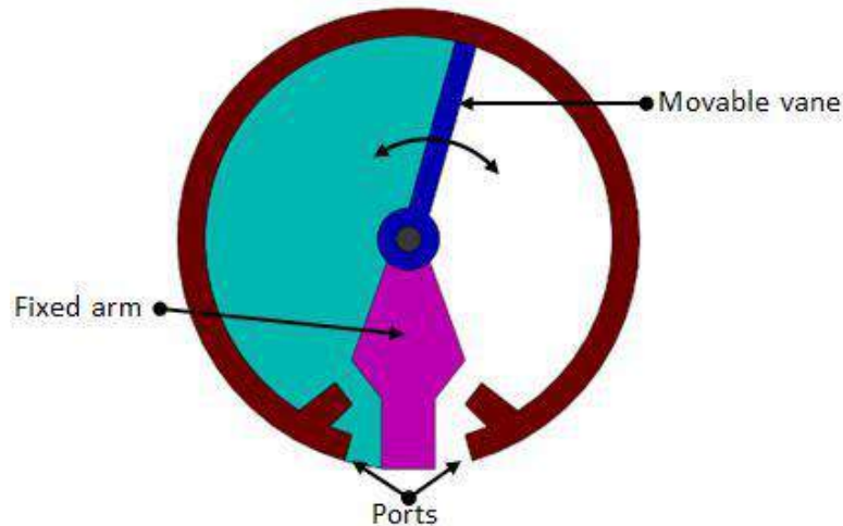
Fig. 5.3.6 Semi rotary vane type actuator
