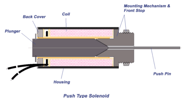
Fig 4.7.1: Solenoid
